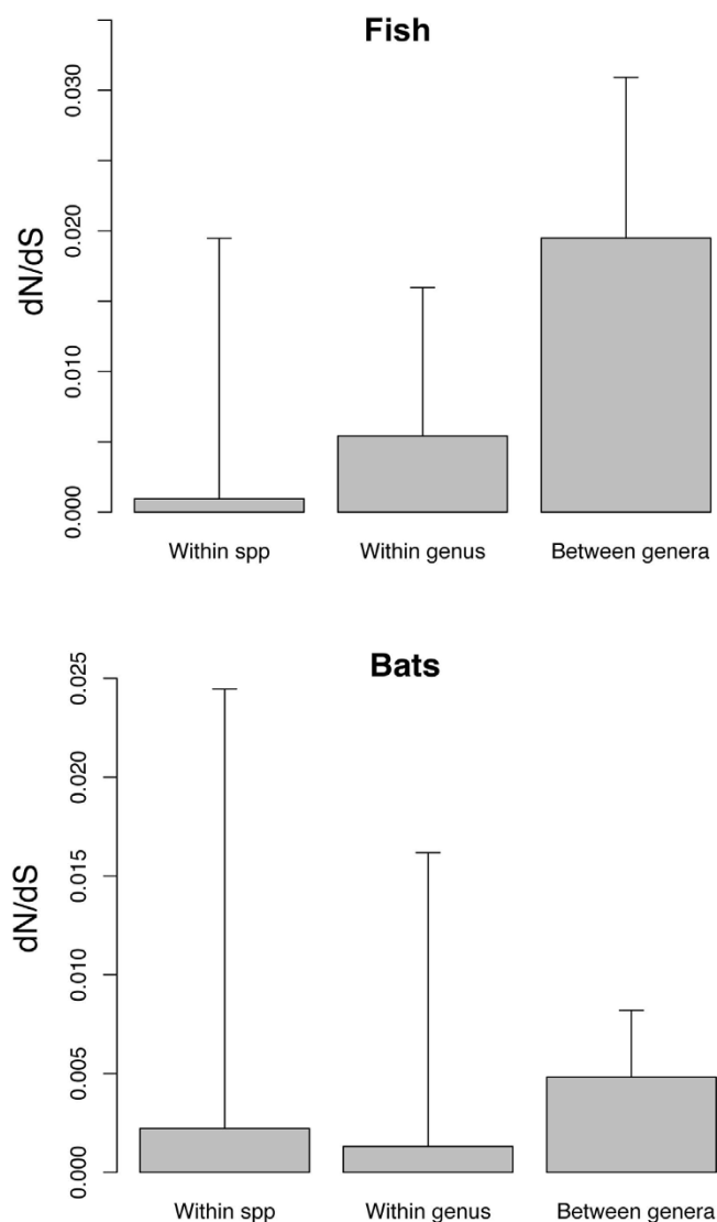
Figure 3 Test of selection at different taxonomic levels. Bar graphs representing the ratio of non-synonymous to synonymous nucleotide substitutions ( \omega ) within species, within genus, and between genera for two exemplar data sets of fish [4] and bats [20].
